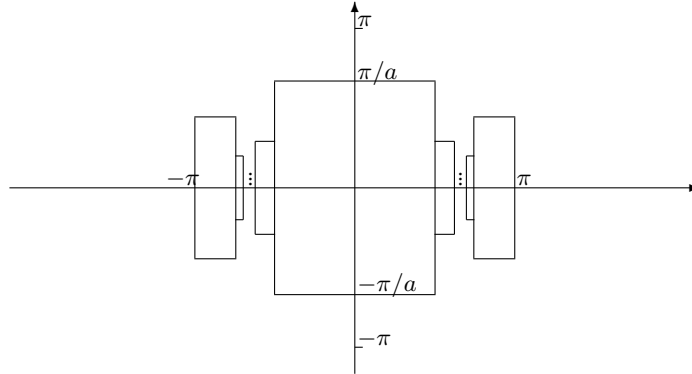
FIGURE 2. The set K .
