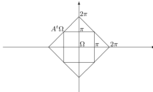
FIGURE 1. The set E = A^t\Omega \setminus \Omega
