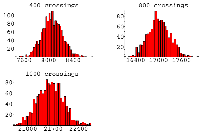
Figure 12. The embedding length distributions of the 1601 400-crossing prime knots, 1092 800-crossing prime knots and 1446 1000-crossing prime knots. The x -axis shows the embedding length and the y -axis shows the frequency of occurrences.
