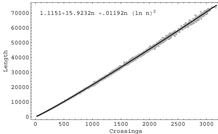
Figure 11. The length data of 2790 knots with crossing numbers ranging from 25 to 3174 together with the plot of the function y = 1.1151 + 15.9232n + 0.01192n \ln^2 n .
