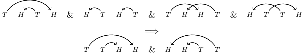
FIGURE 3. A graphical representation of the first case of Proposition 3.8.
