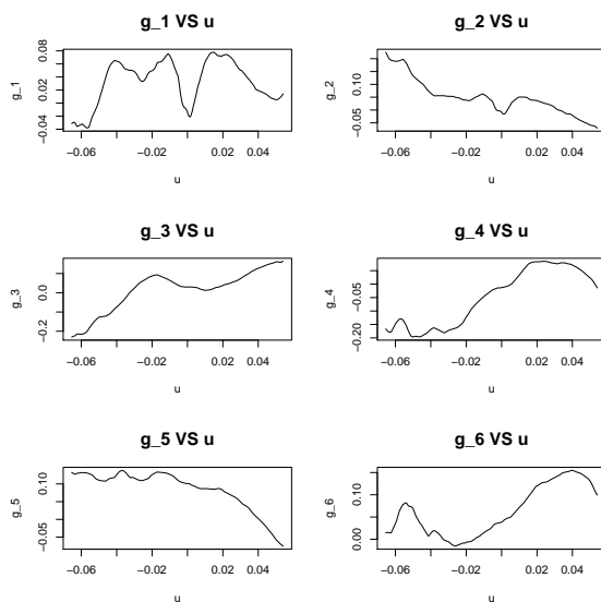
Figure 2.6: Non-zero functional coefficient for FIAR with weekly NASDAQ data
