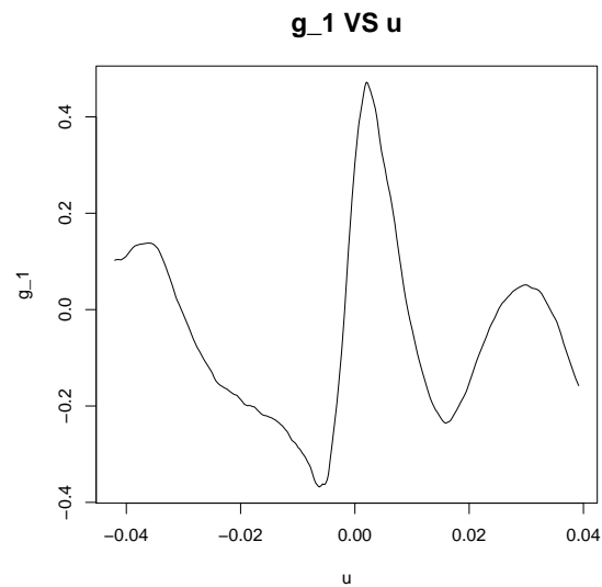
Figure 2.5: Non-zero functional coefficient for FIAR with weekly DOW data
