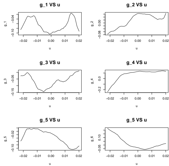
Figure 2.2: Non-zero functional coefficient for FIAR with daily DOW data
