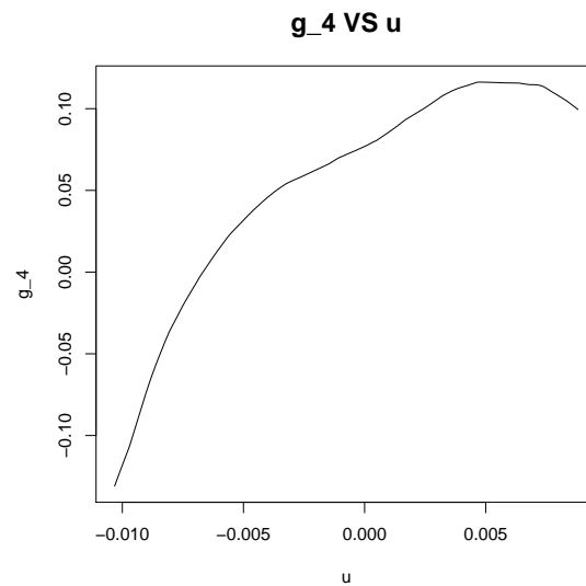
Figure 2.3: Non-zero functional coefficient for FIAR with daily NASDAQ data
