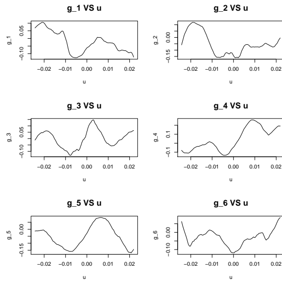
Figure 2.4: Non-zero functional coefficient for FIAR with daily SP data
