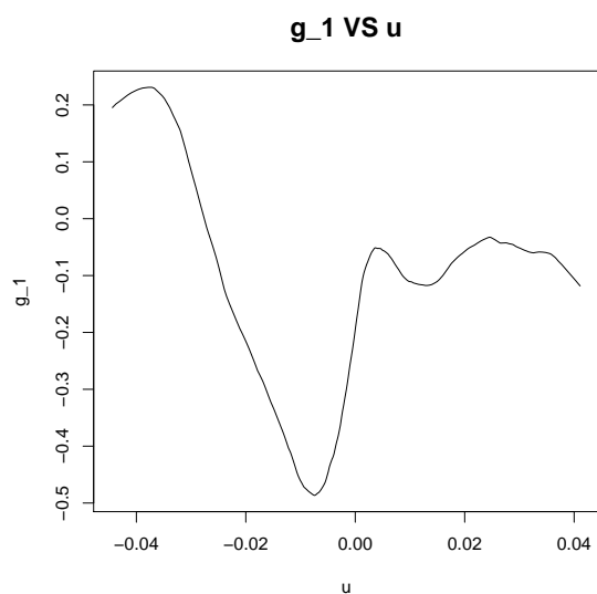
Figure 2.7: Non-zero functional coefficient for FIAR with weekly SP data
